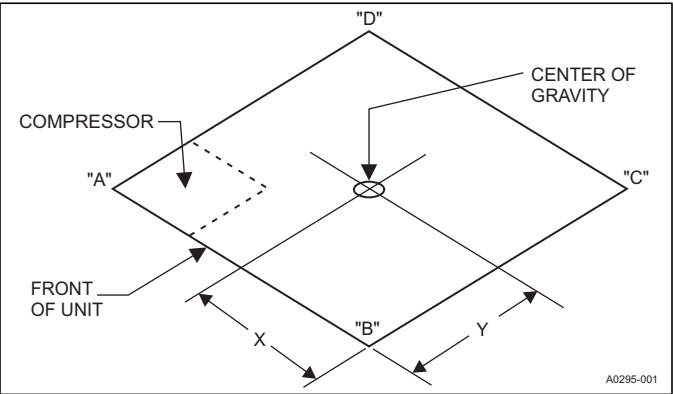
FIGURE 2: Unit 4 Point Load Weight
