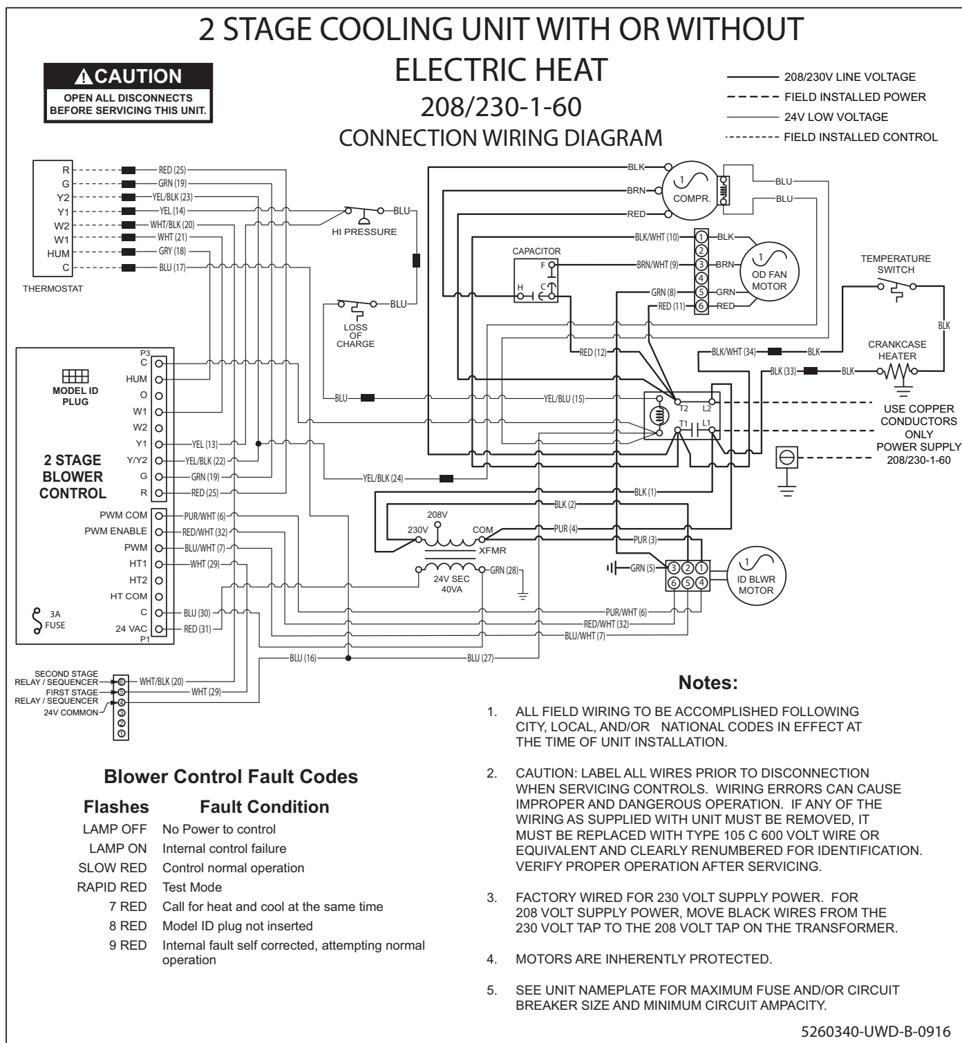
FIGURE 11: Connection Wiring Diagram
