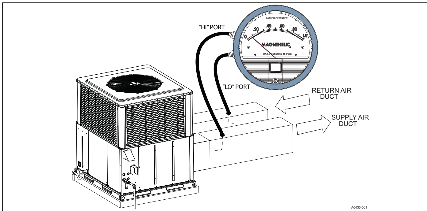
FIGURE 10: Measuring External Static Pressure
