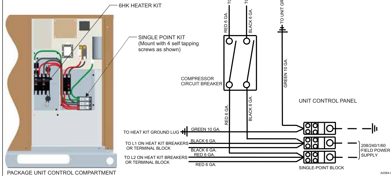
FIGURE 8: Single-point Wiring Kits
